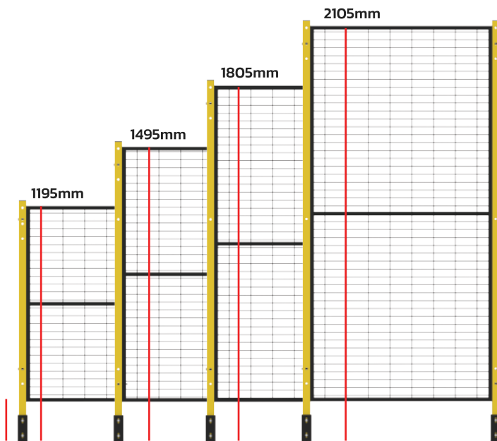
Floor to panel clearance 205mm
